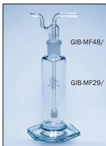
Dreschel Bottle & Sintered Head
